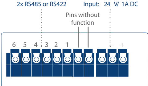
Fig.: Top Connections – Gateway Solar-Log 50
